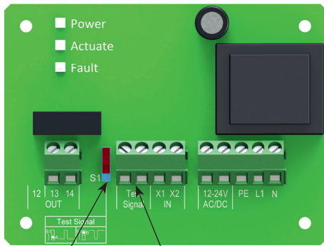
DIP slide switch S1 Test signal connection terminals
