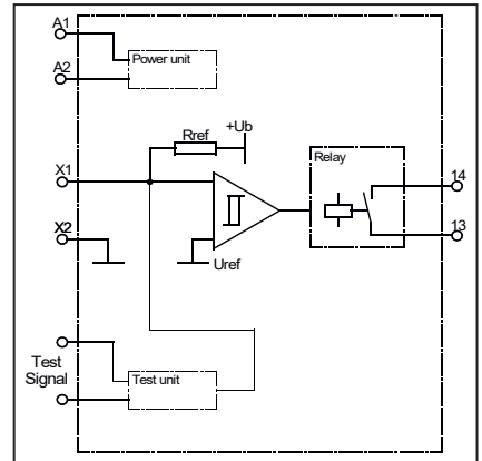
Simplified diagram ELMON relay 31-30
